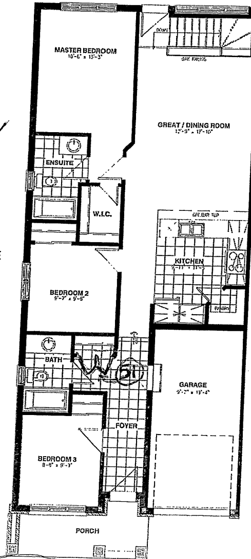
GROUND FLOOR STANDARD 3 BEDROOM PLAN
