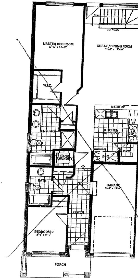
GROUND FLOOR OPTIONAL 2 BEDROOM PLAN
