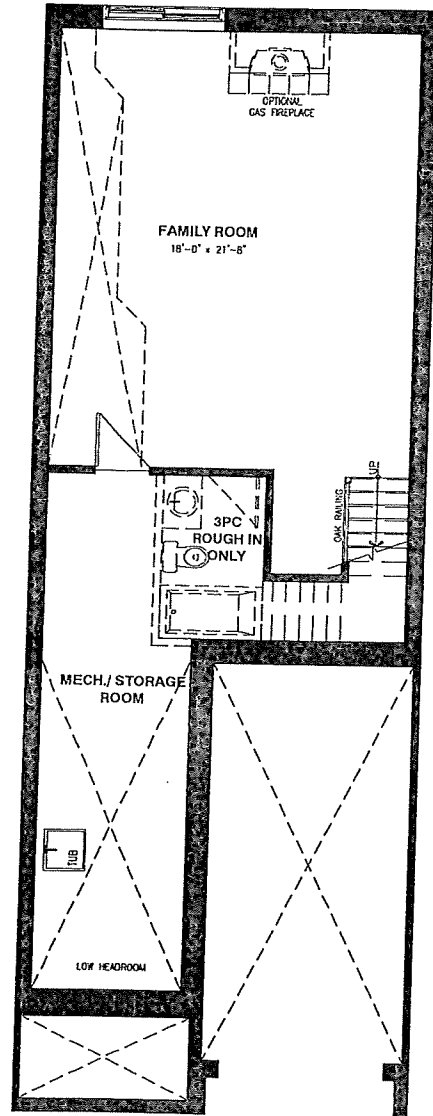
BASEMENT FLOOR
