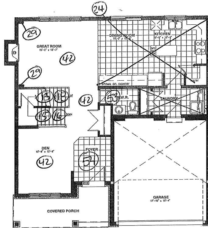
GROUND FLOOR - ELEVATION A & B
