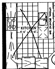
OPTIONAL KITCHEN #1
