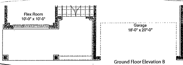
Ground Floor Elevation B
