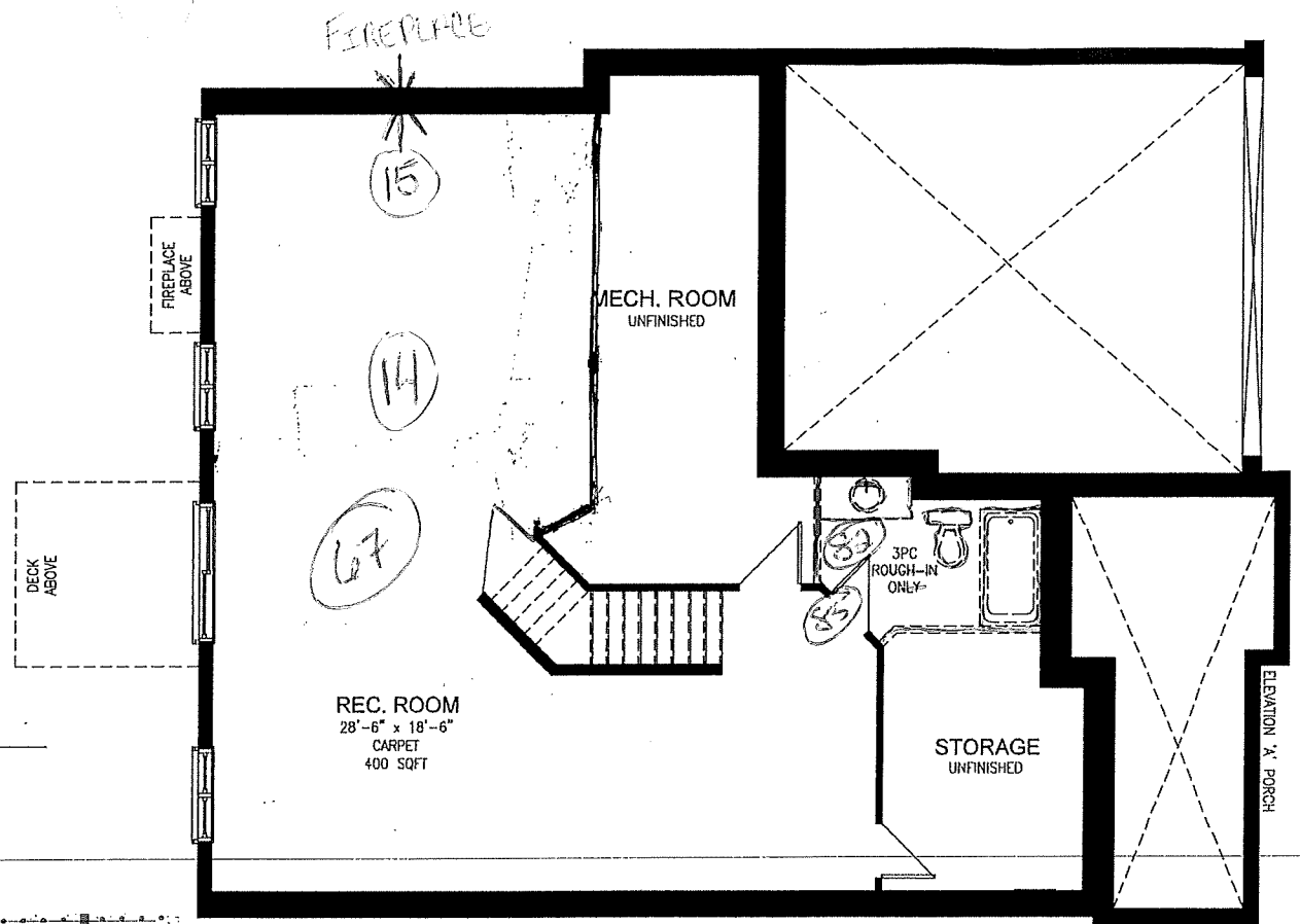
WALKOUT BASEMENT PLAN
