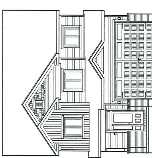
ELEVATION C
