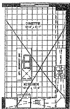
OPTIONAL KITCHEN #3
