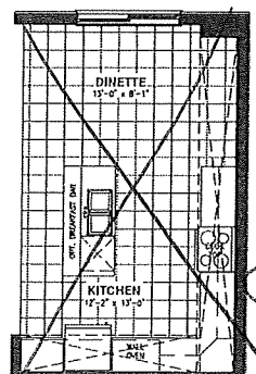
OPTIONAL KITCHEN #3
