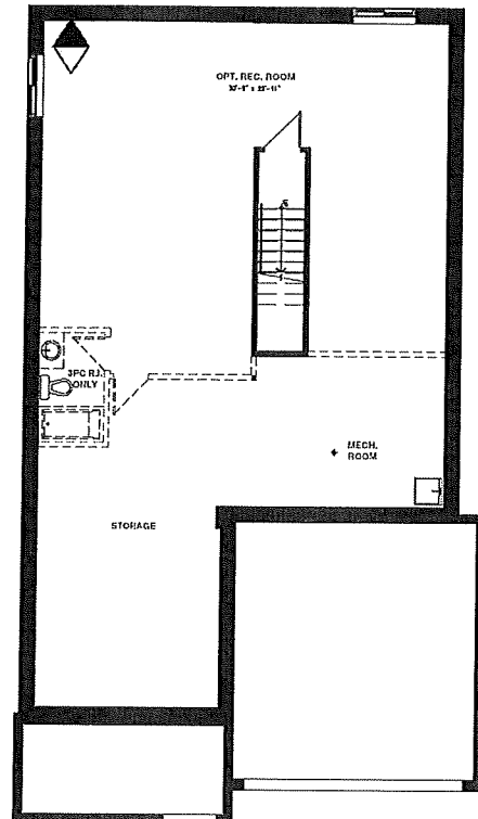
BASEMENT FLOOR - ELEVATION A
