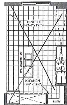
OPTIONAL KITCHEN #1
