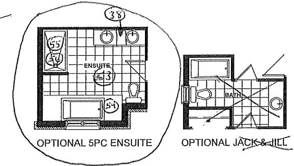
SECOND FLOOR - 4 BEDROOMS - ELEVATION A
