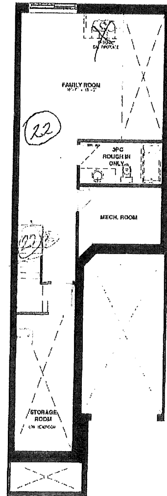
BASEMENT FLOOR
