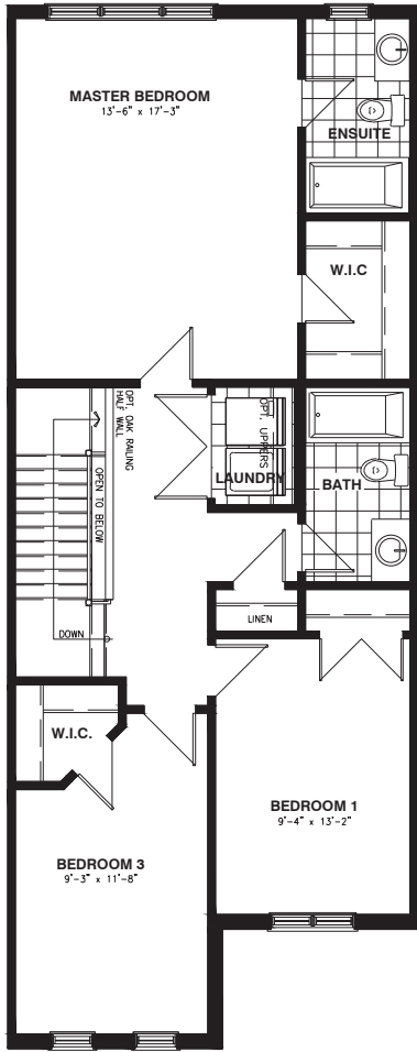
SECOND FLOOR
