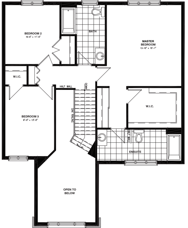
SECOND FLOOR ELEVATIONS A & C
