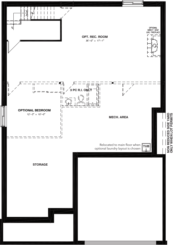
BASEMENT FLOOR - ELEVATION A & B
