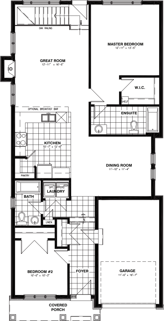
GROUND FLOOR A
