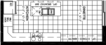
Optional Kitchen #2
