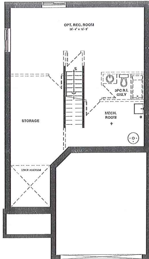
BASEMENT FLOOR
