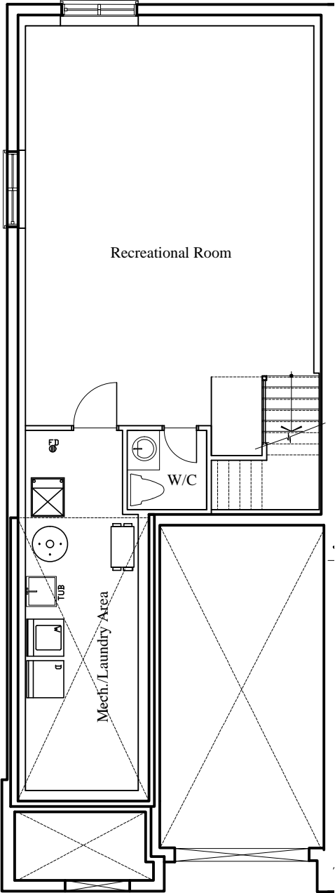
BASEMENT FLOOR
