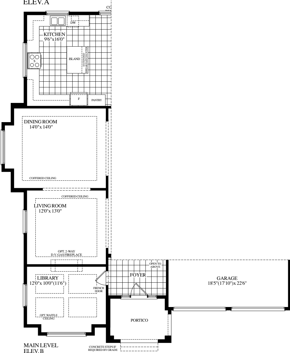
MAIN LEVEL ELEV. B
