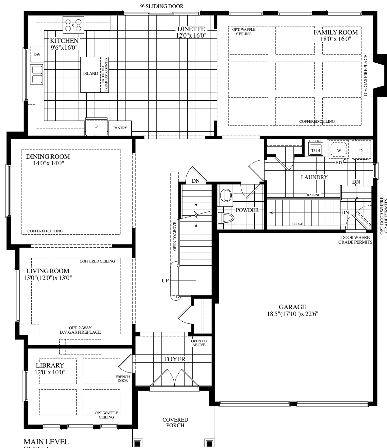
MAIN LEVEL ELEV.A
