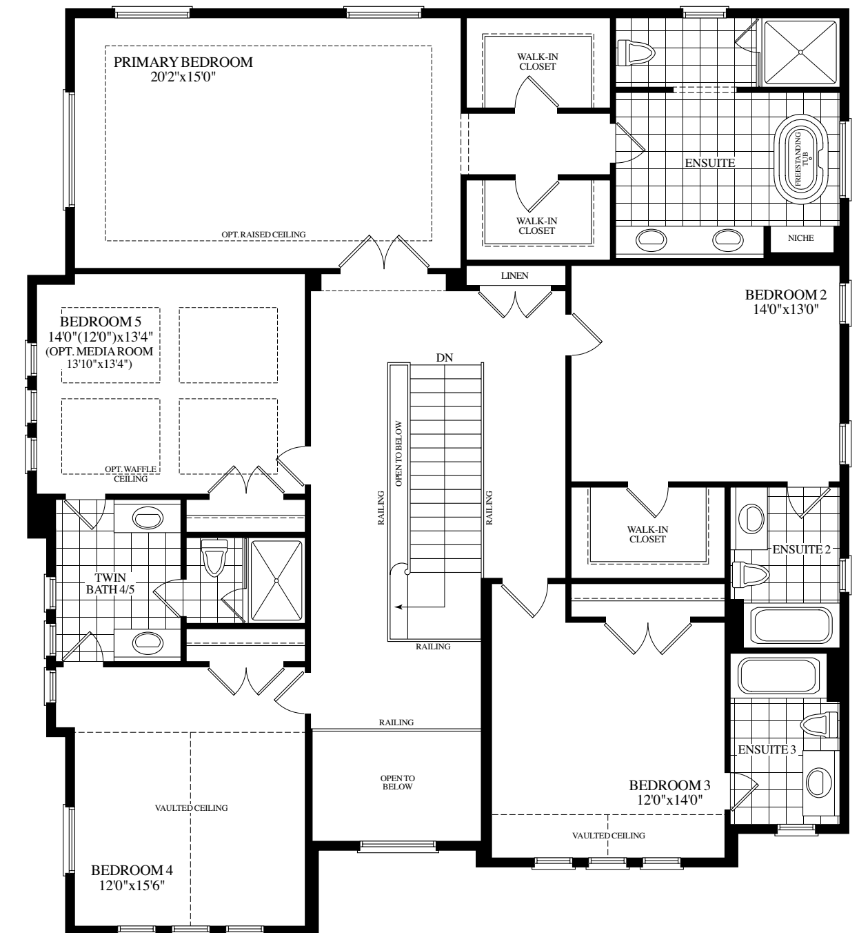
OPT. UPPER LEVEL ELEV.A
