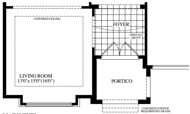
MAIN LEVEL ELEV. B
