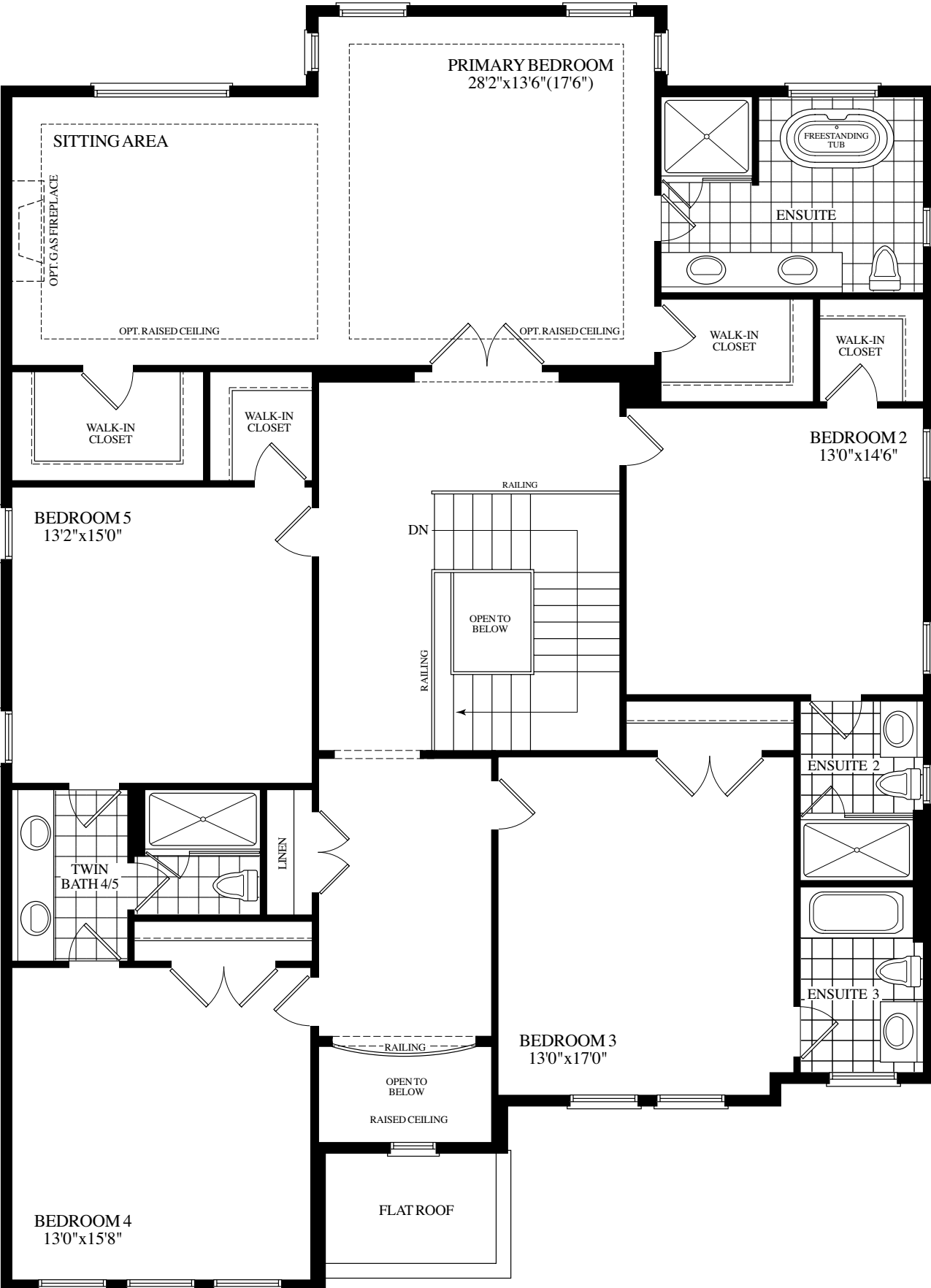
UPPER LEVEL ELEV. A
