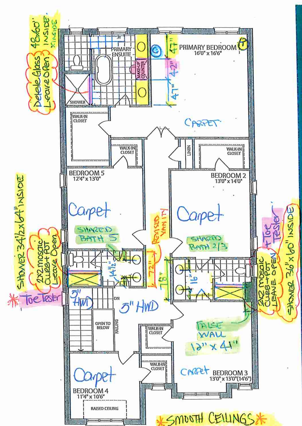
SECOND FLOOR ELEV. A
