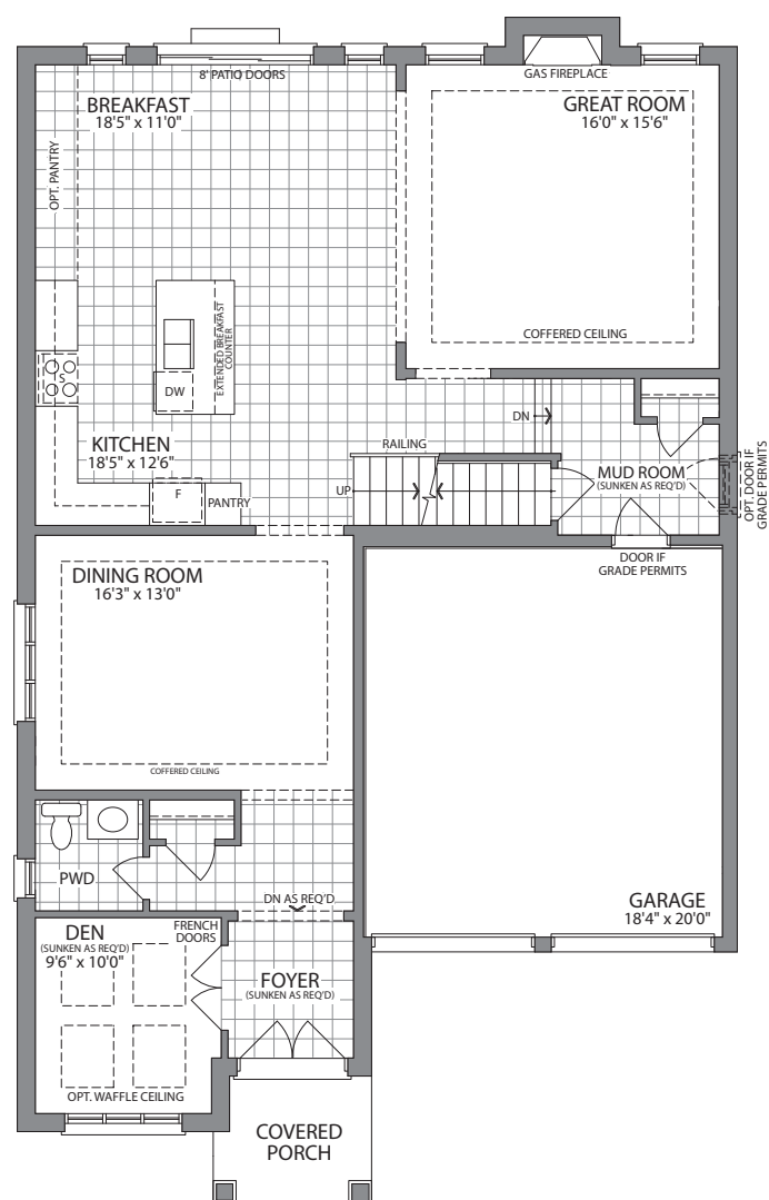
OPT. GROUND FLOOR ELEV. A
