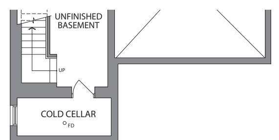
BASEMENT ELEV. B
