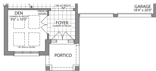
OPT. GROUND FLOOR ELEV. B
