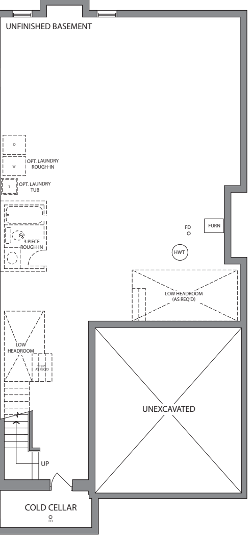
BASEMENT ELEV. A & B
