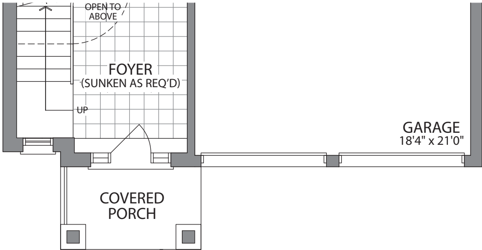
GROUND FLOOR ELEV. C
