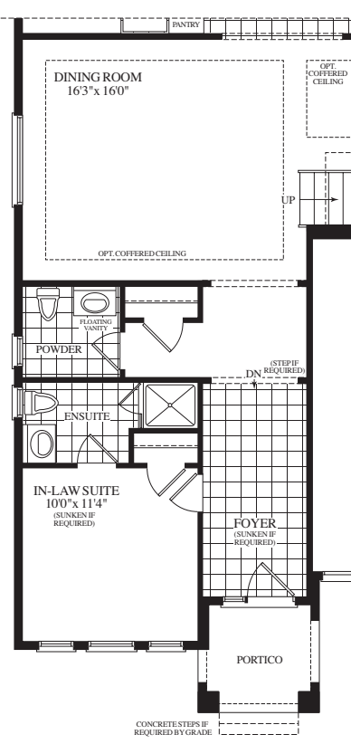
PART MAIN LEVEL WITH IN-LAW SUITE ELEV. A
