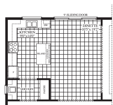
PART MAIN LEVEL ALTERNATE KITCHEN LAYOUT ELEV. A & B
