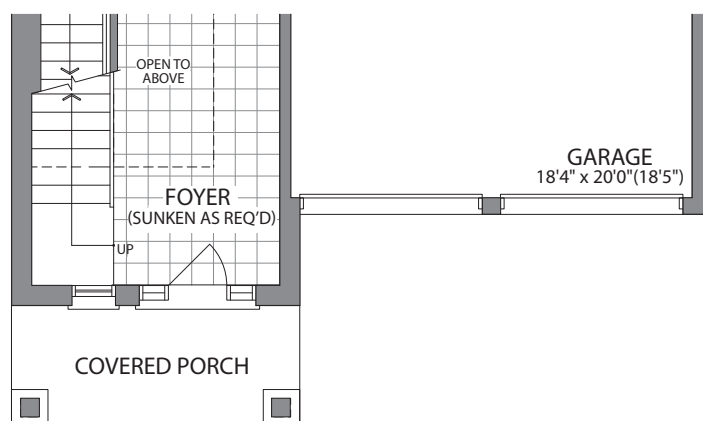
GROUND FLOOR ELEV. C
