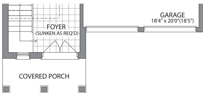
GROUND FLOOR ELEV. B
