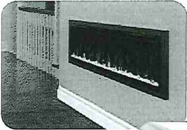
50" IgniteXL Trim Kit (XLFTRIM50) Allows installation of IgniteXL in 2"x4" wall construction. 52-3/4" x 18-1/4" x 1-7/8" (134.0 cm x 46.2 cm x 4.5 cm)
