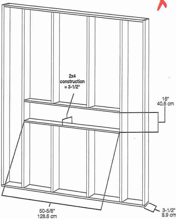
2x4 framing
