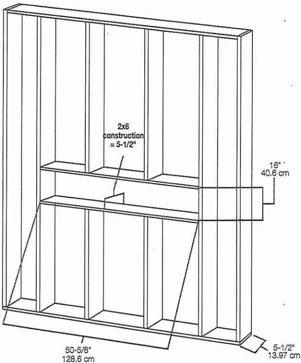
2x6 framing
