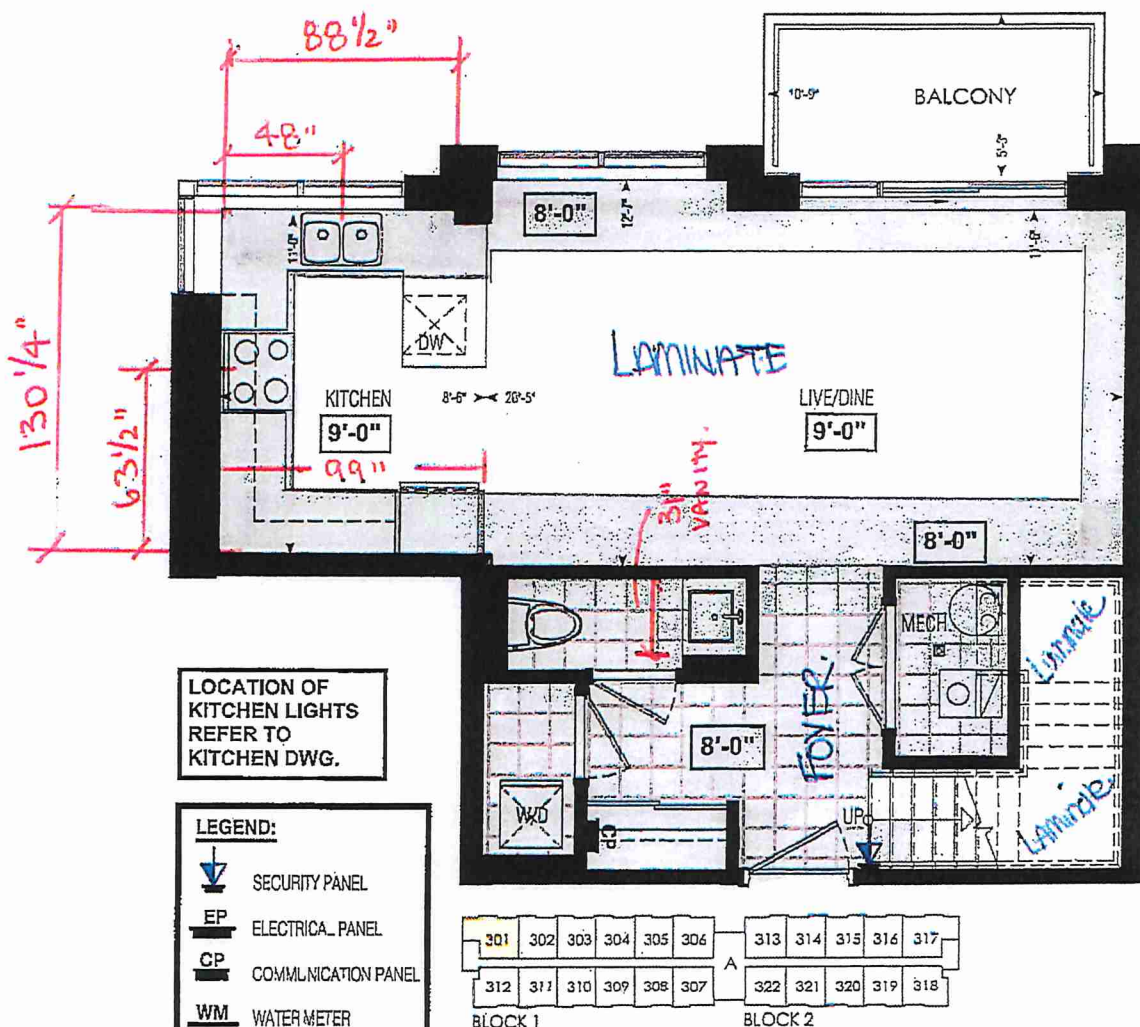
THIRD FL.
