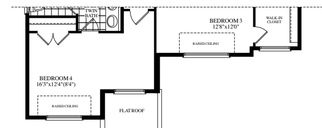
OPT. UPPER LEVEL ELEV. A (5 BEDROOM & 4 BATH)
