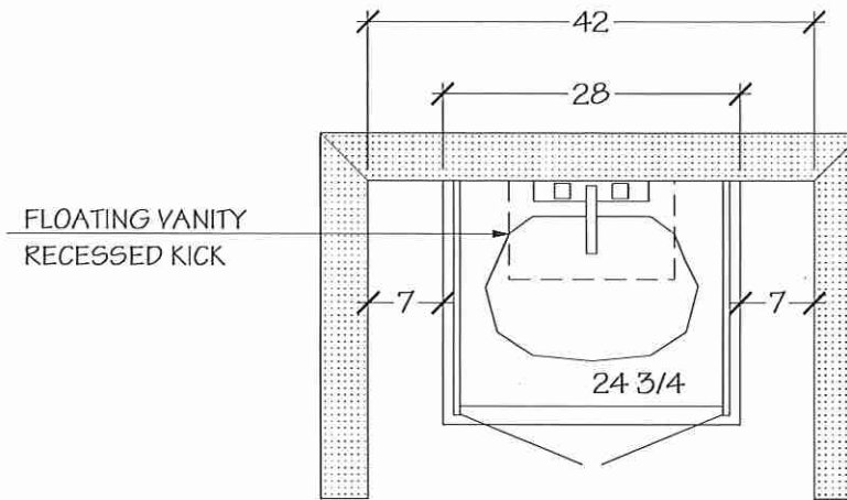
POWDER ROOM
