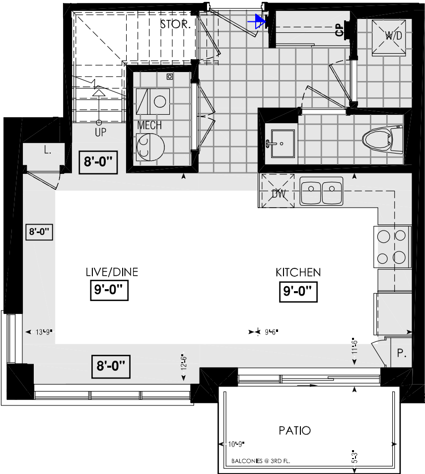
FOURTH FL.
