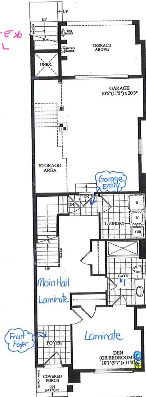
GROUND LEVEL ELEV.A
