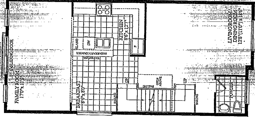
MAIN LEVEL ELEV. A & B
