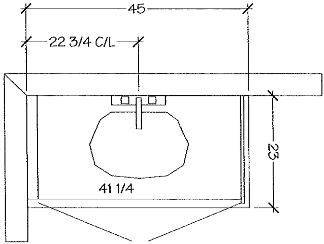
MAIN BATH
