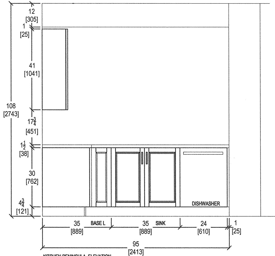
KITCHEN PENINSULA ELEVATION FRONT VIEW
