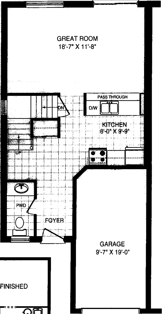
Main Floor
