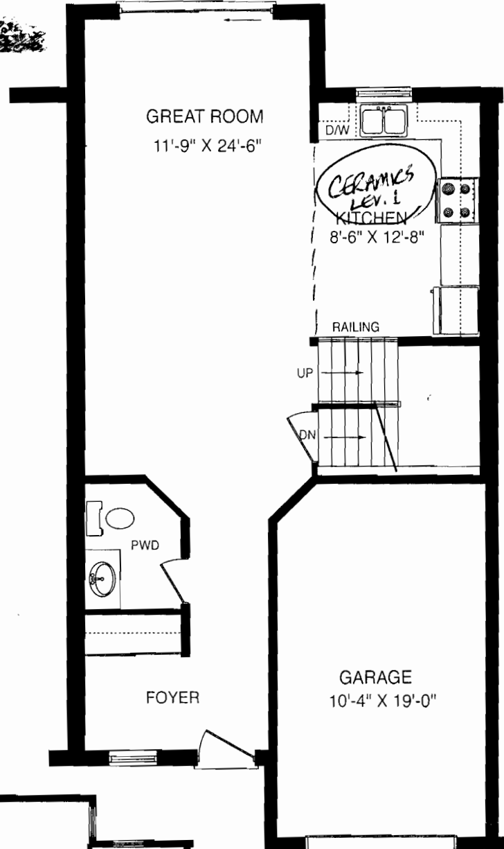
Main Floor
