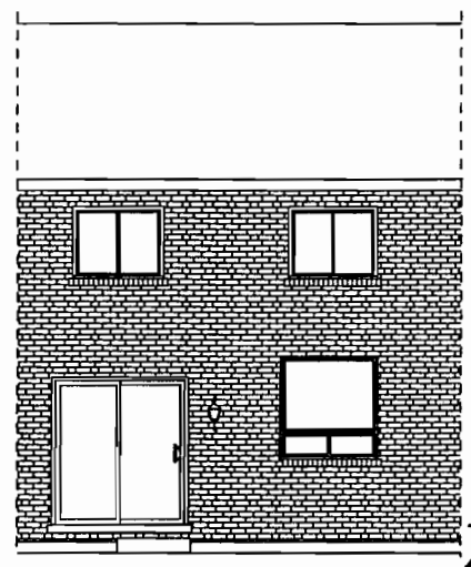
Back Elevation
