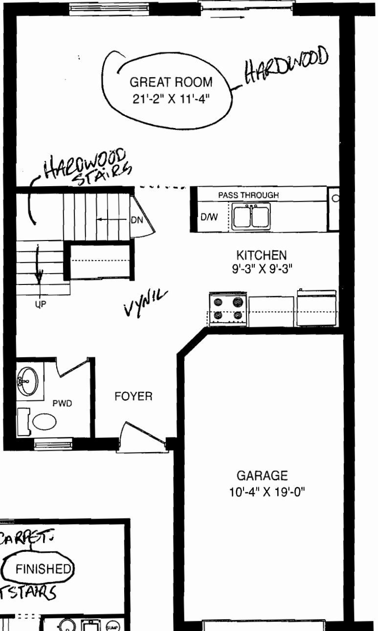
Main Floor
