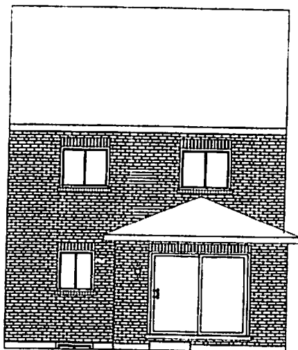
Back Elevation
