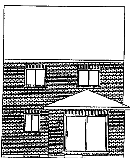
Back Elevation
