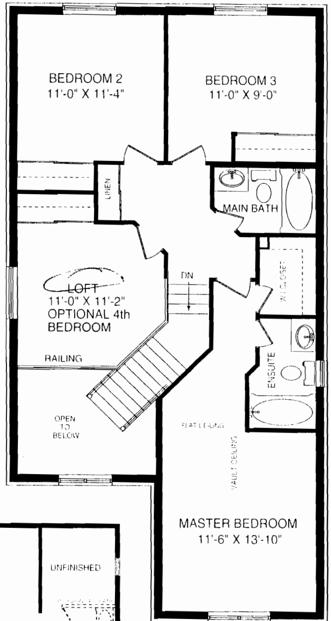
Second Floor
