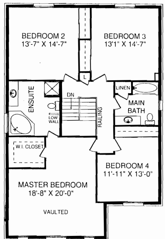
Second Floor 4 Bedroom
