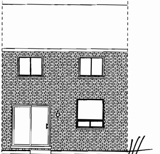
Back Elevation
