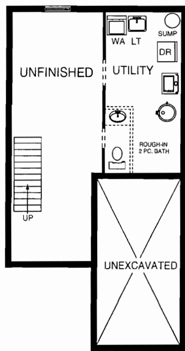
Basement
