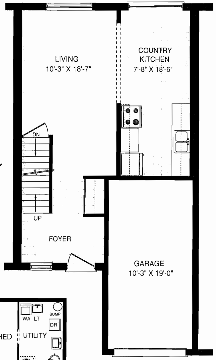
Main Floor
