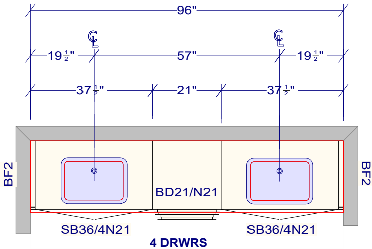
KITCHEN HEIGHT CABINETS SHARED BATH BDRM 3 & 4
