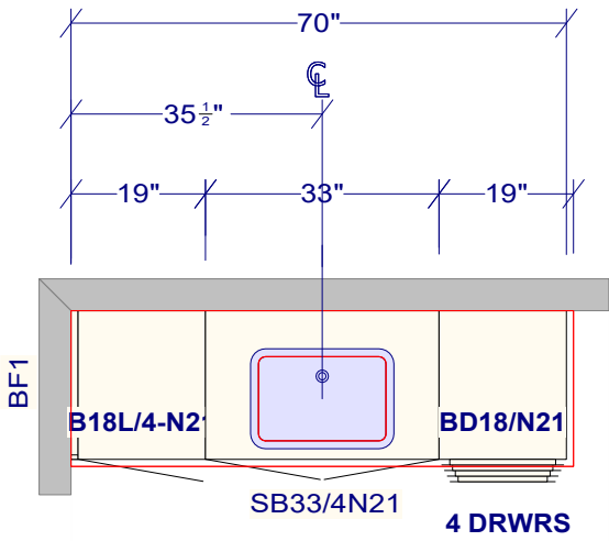
KITCHEN HEIGHT CABINETS ENSUITE #2
