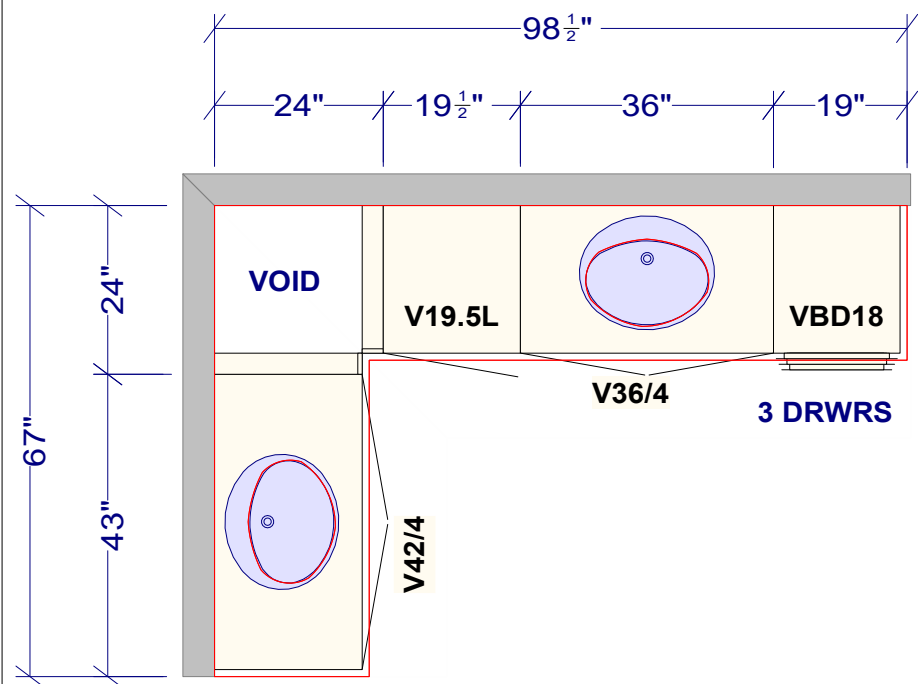
PRIMARY ENSUITE
