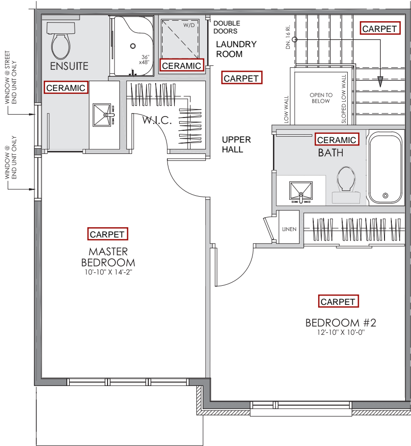
FLOOR LAYOUT AND TILE PATTERN JUN B8 UNIT 248 / CIVIC 619
