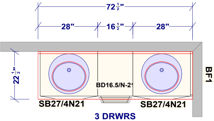
MAIN BATH
