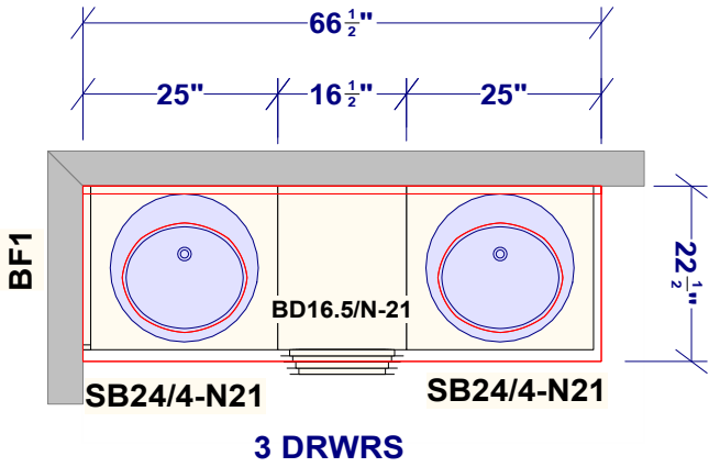
PRIMARY ENSUITE
