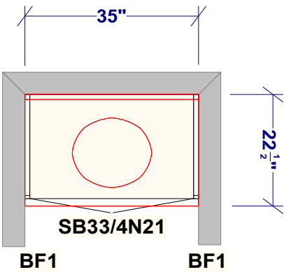
POWDER ROOM
