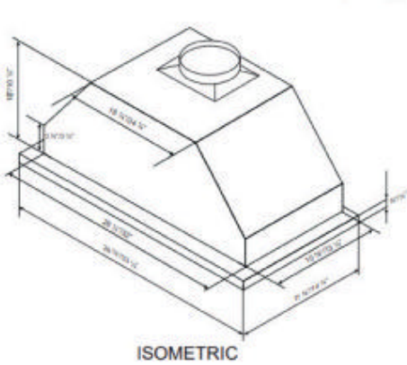
ISOMETRIC
