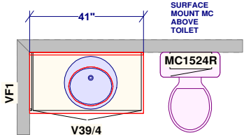
MAIN BATH
