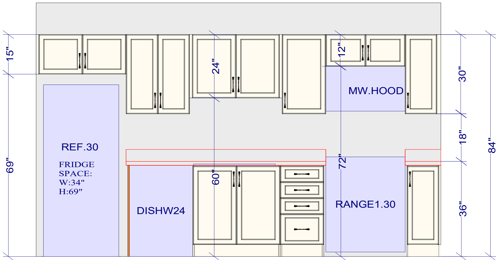
FRIDGE / RANGE WALL ELEVATION
